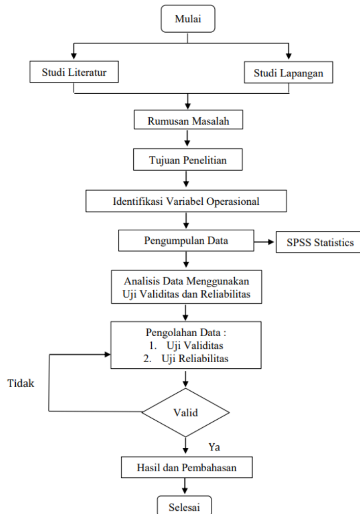
Gambar 1. Flowchart
